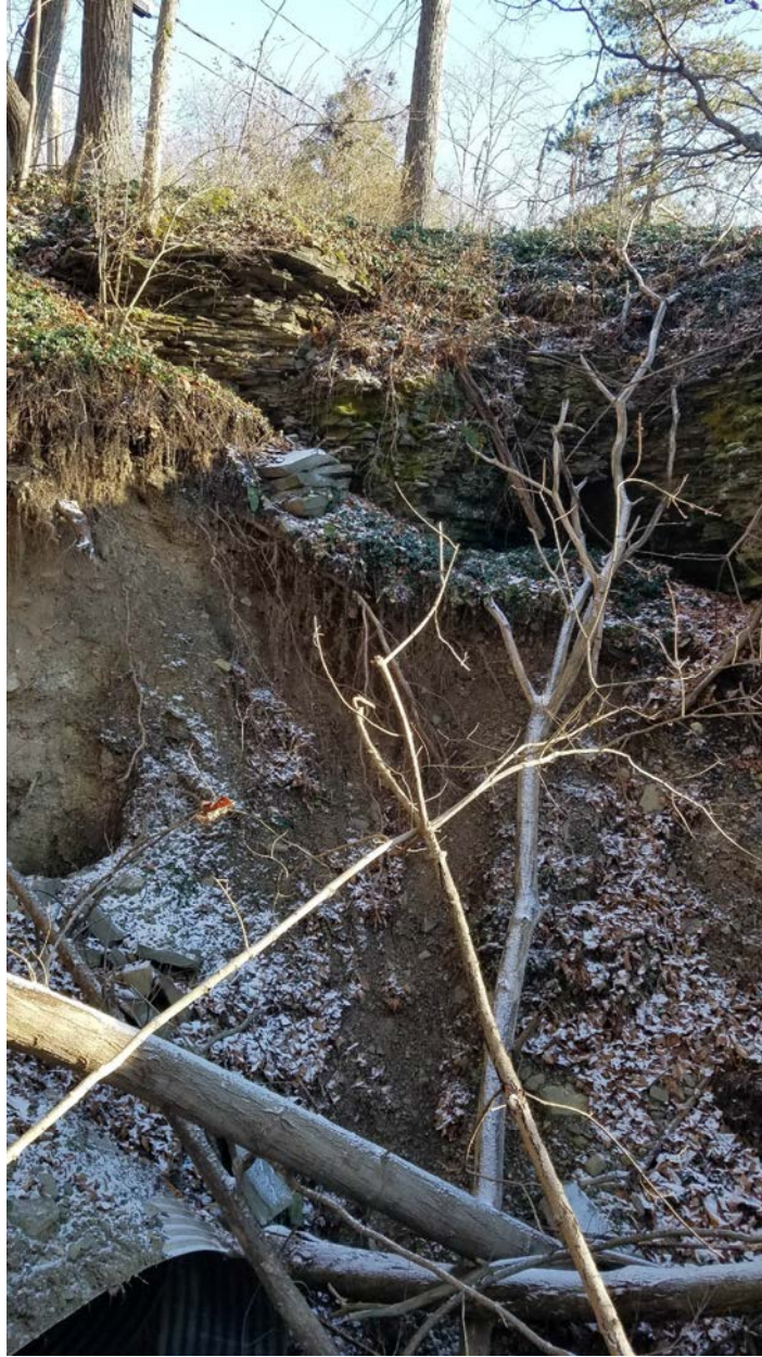
Photo #5 – Outlet End – Erosion of surrounding area near pipe separation in Photo #4
